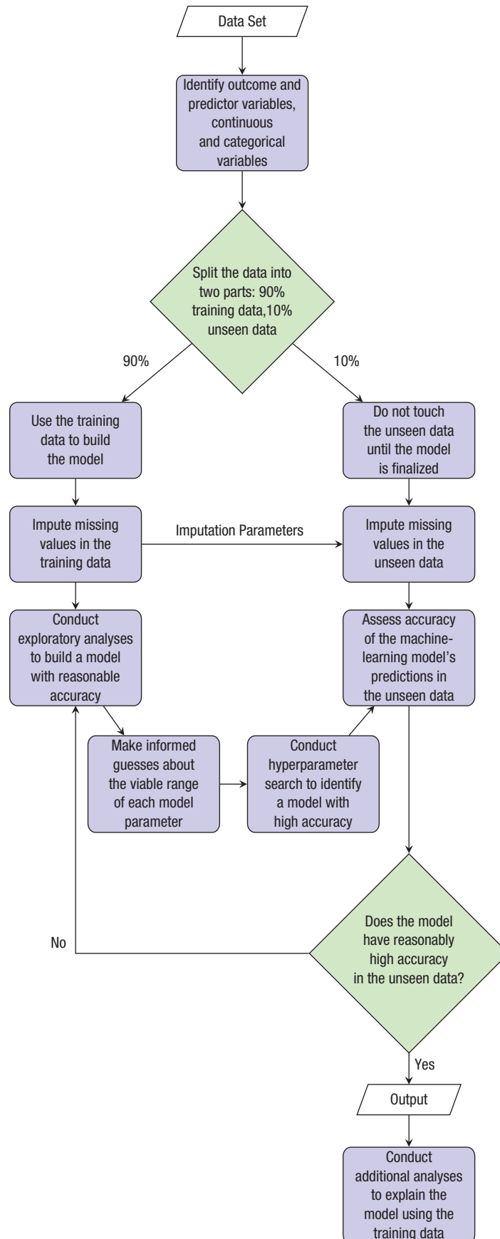
Fig. 1. Flowchart showing the machine-learning procedure used in Study 1.
