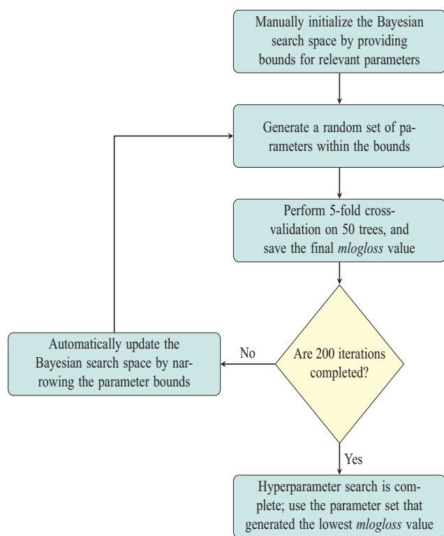
Figure 2 Illustration of the Bayesian Hyperparameter Search Procedure
