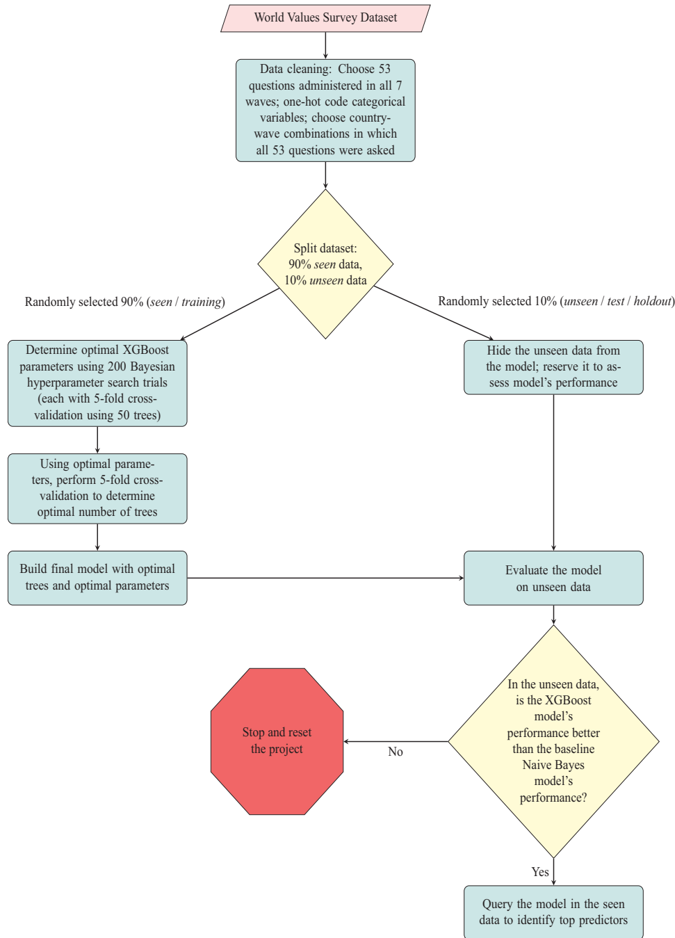
Figure 1 Illustration of the Machine Learning Procedure
